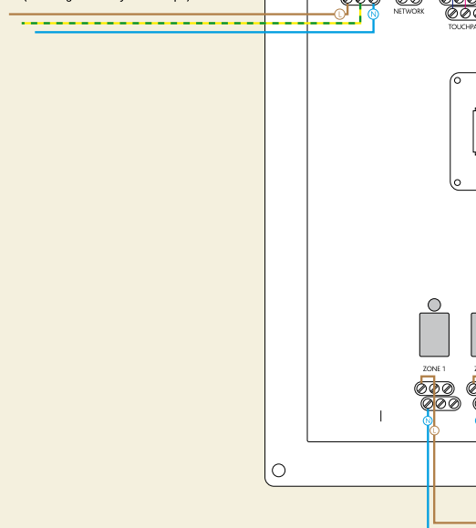
230V AC Supply (Via Heating/Hot Water System Fused Spur)
